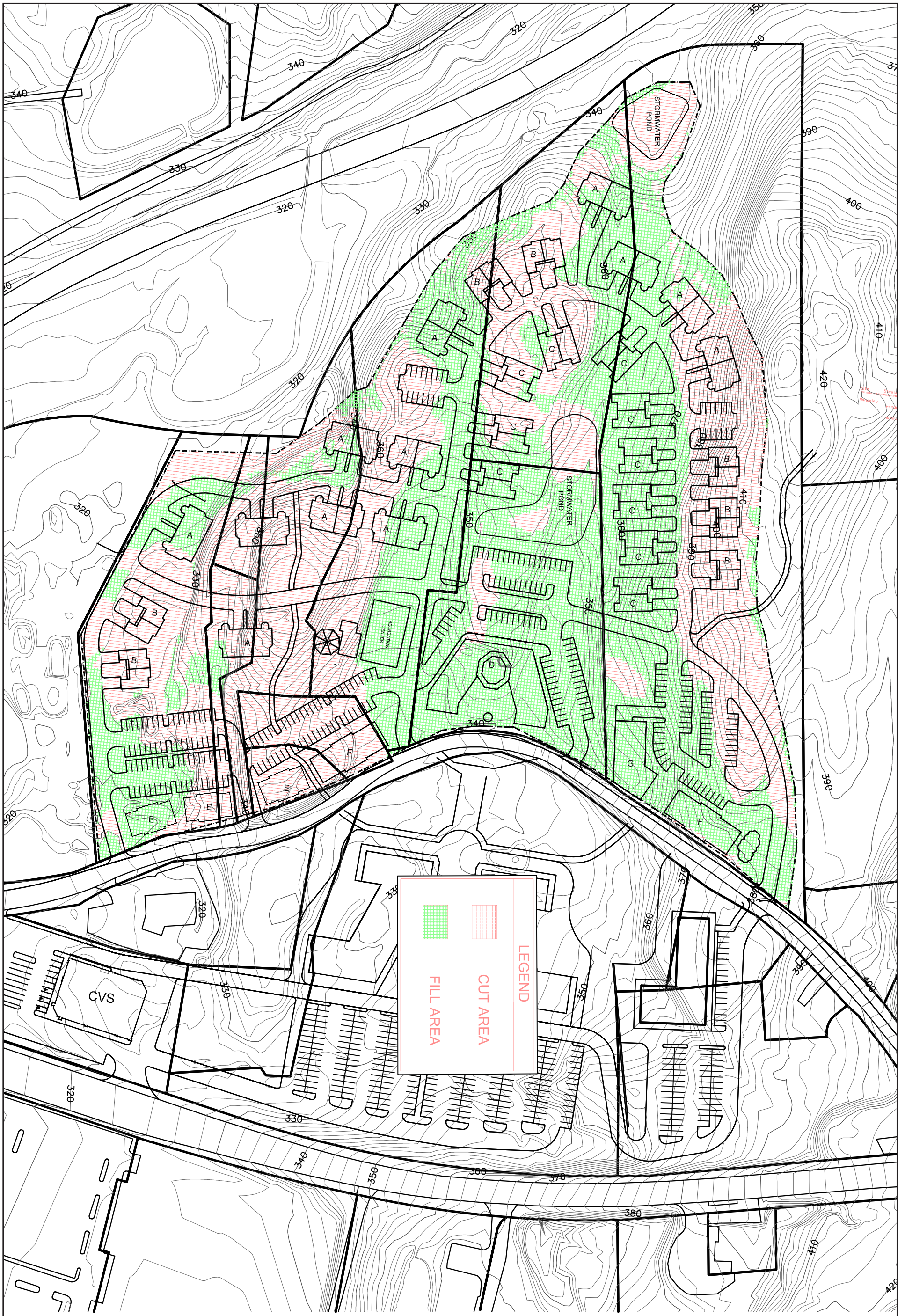
Figure 4-4: Preliminary Earthwork Estimate Bear Mountain Triangle Rezoning Town of Yorktown, New York Source: Ciarcia Engineering, P.C. Approx. Scale: 1" = 150'
